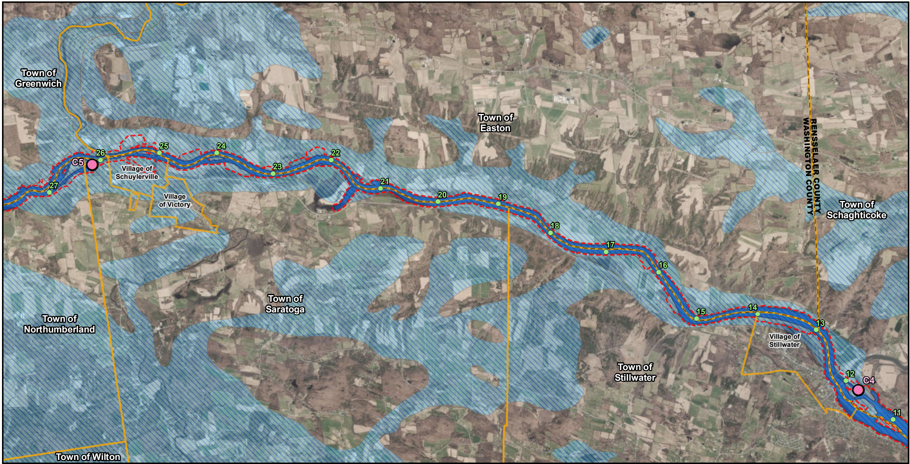
Figure 12F: Aquifers
